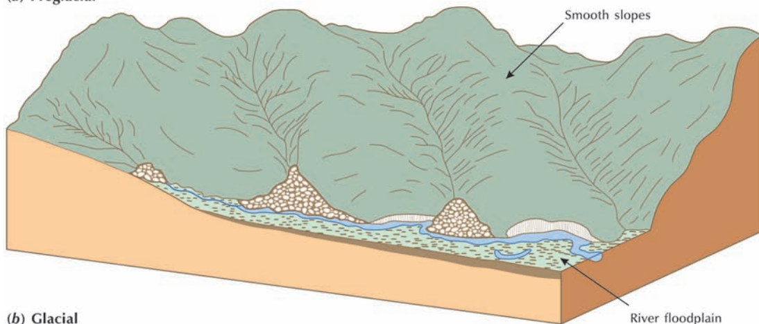
(b) Glacial
