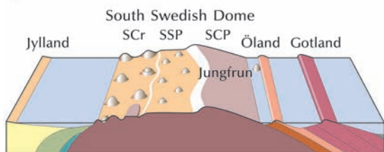
(g) Present
