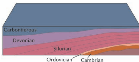
(b) Cambrian–Carboniferous
