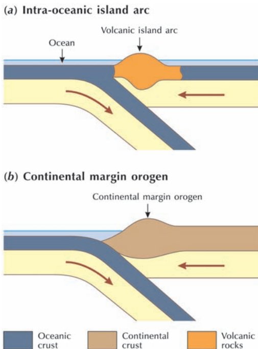
Figure 5.11 The two kinds of steady-state margins. (a) Intra-ocean island arc formed where an oceanic plate is subducted beneath another oceanic plate. These are common in the western Pacific Ocean. (b) A continental margin orogen formed where an oceanic plate is subducted beneath a continental 'plate'. An example is the Andes. Source: Adapted from Summerfield (1991, 58)
