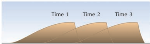
Figure 12.5 The downwind progress of a transverse dune. Source: Adapted from Livingstone and Warren (1996, 73)
