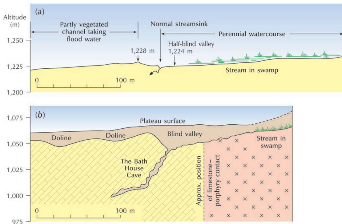
Figure 14.11 Blind and half-blind valleys in New South Wales, Australia. (a) A half-blind valley on Cooleman Plain. (b) A blind valley at Yarrangobilly. Source: Adapted from Jennings (1971, 110, 111)
