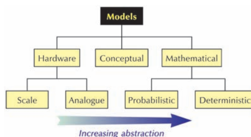
Figure 2.8 Types of model in geomorphology. Source: After Huggett (1993, 4)
