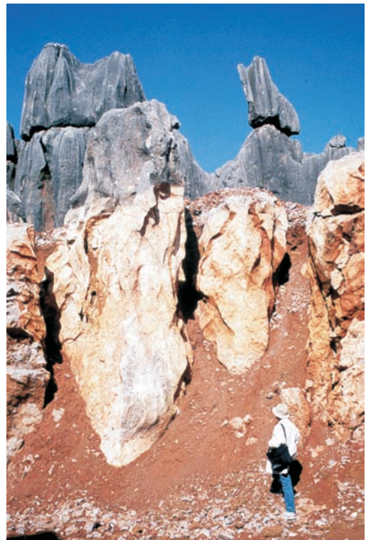
Plate 14.5 Pinnacle karst or shilin (shilin means 'stone forest' in Mandarin) exposed in a road-cut in Shilin National Park, Yunnan, China. The subsoil origin of the pinnacles is plainly seen. Their emergence is due to the general erosion of regional cover sediment. (Photograph by Derek C. Ford)
