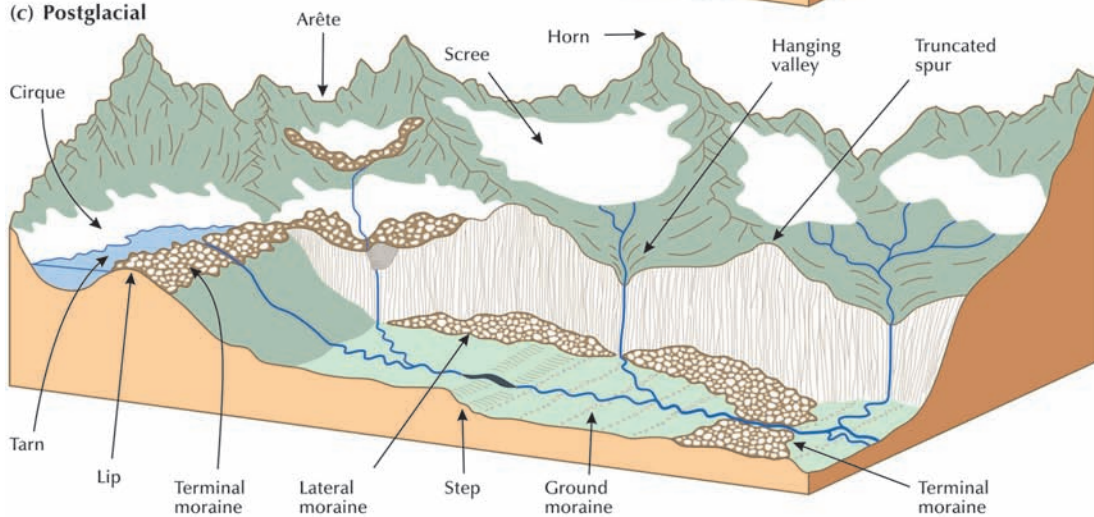
(c) Postglacial
