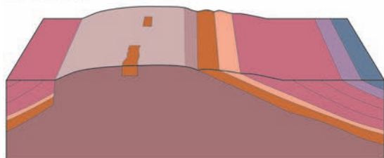
(c) Permian
