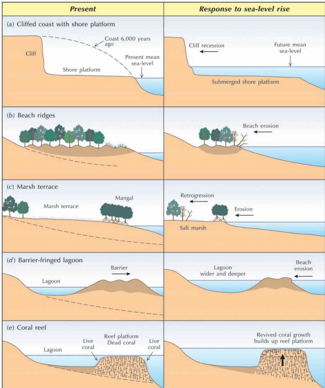
Figure 13.22 Coastal changes brought about by a rising sea level. (a) Clifed coast with shore platform. (b) Beach ridges. (c) Marsh terrace. (d) Barrier-fringed lagoon. (e) Coral reef. Source: Adapted from Bird (2000, 278)
