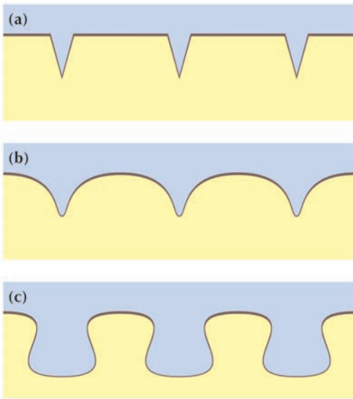
Figure 14.16 Proposed sequence of events leading to 'bollar' rock formation in quartzitic sandstone, north-central Thailand. (a) Polygonal cracks develop in a case-hardened surface that act as avenues of weathering. (b) Weathering deepens the cracks, forming a convex surface on each polygonal block. (c) Further weathering removes the edges of the polygonal blocks and deepens and widens the cracks. Source: Adapted from Robinson and Williams (1992) and Doerr (2000)
