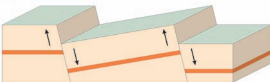
Figure 6.19 Up-faulted structures. (a) Horst. (b) Tilted block.
