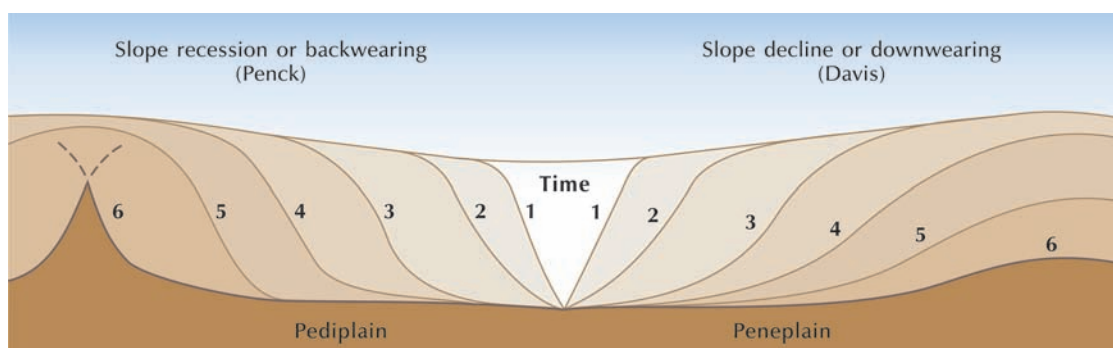
Figure 15.1 Slope recession, which produces a pediplain (p. 439) and slope decline, which produces a peneplain. Source: Adapted from Gossman (1970)
