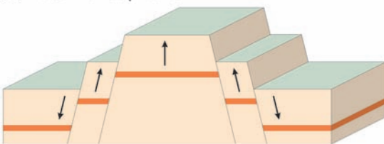
(a) Horst with step faults
