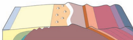
(f) Mid-Miocene–Pliocene
