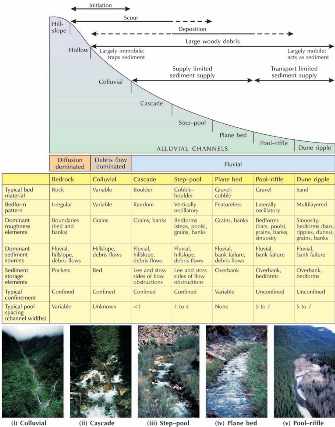
Figure 9.11 Channel forms in mountain streams. Sources: Adapted from Montgomery and Buffington (1997); (Photographs by Dave Montgomery)
