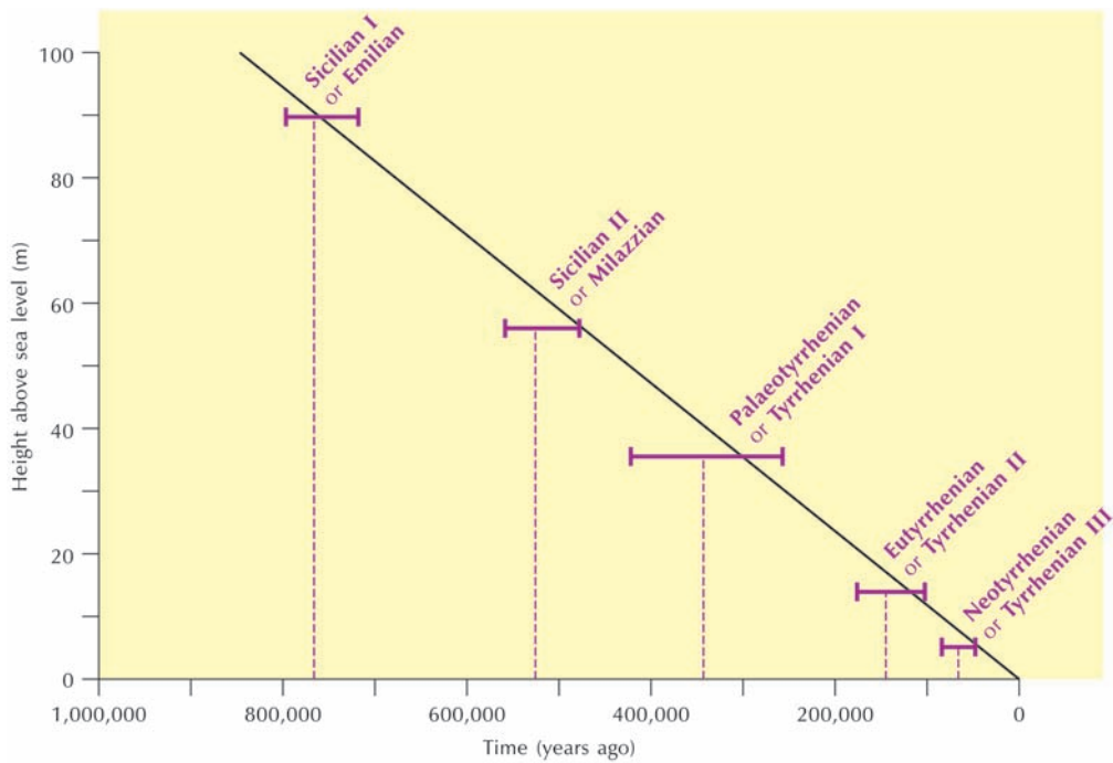
Figure 13.24 Quaternary sea-levels in the Mediterranean: the classic interpretation.
