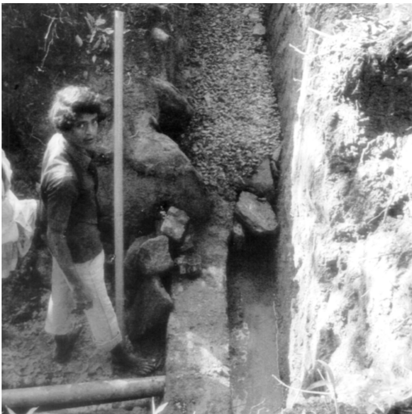
Catchment of contact spring with a “catchment trench”
