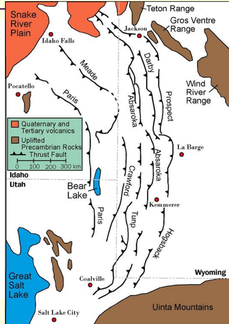
Map of Fold and Thrust Belt redrawn from Armstrong and Oriol (1986).
