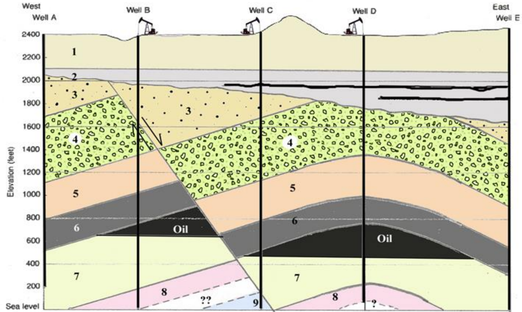
FIGURE 3 Cross section showing well locations.
