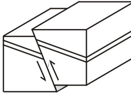
(b) inversa
