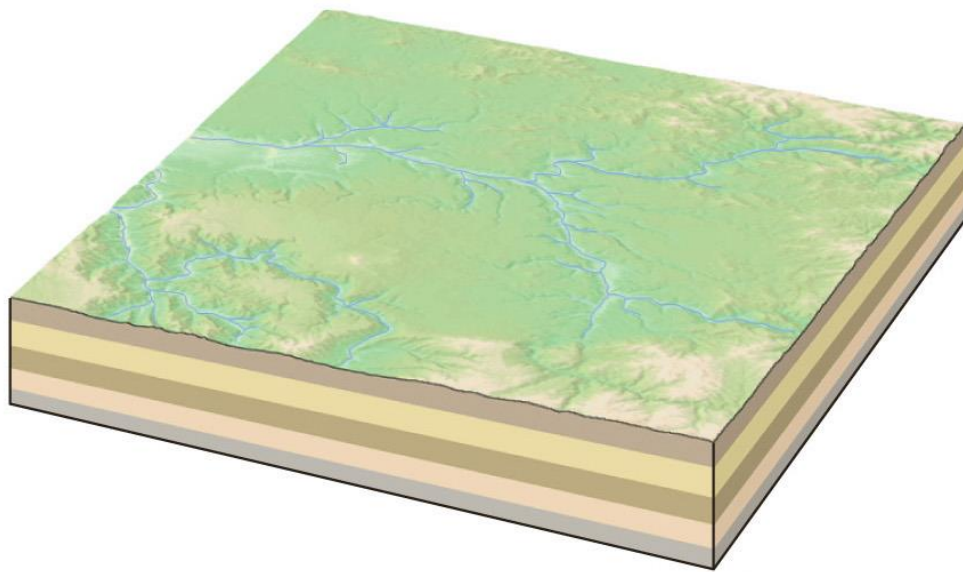
A. Undeformed strata (rock body)
