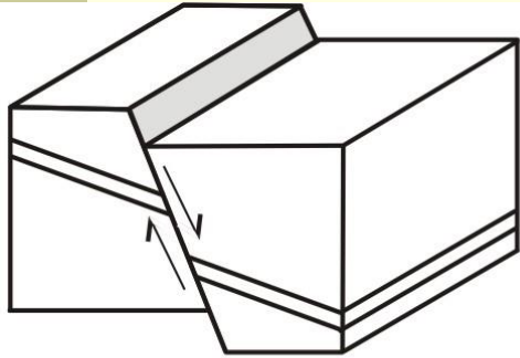
(a) normal
