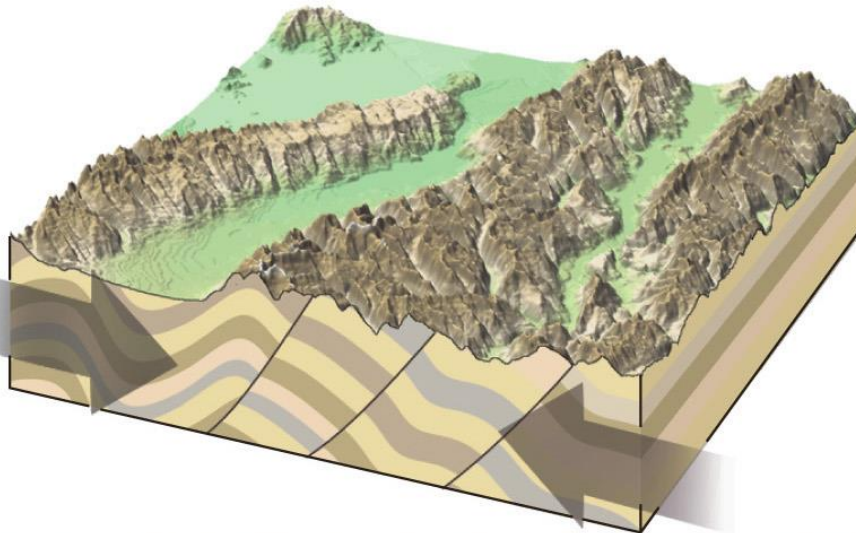
B. Horizontal compressional stress causes rock bodies to shorten horizontally and thicken vertically
