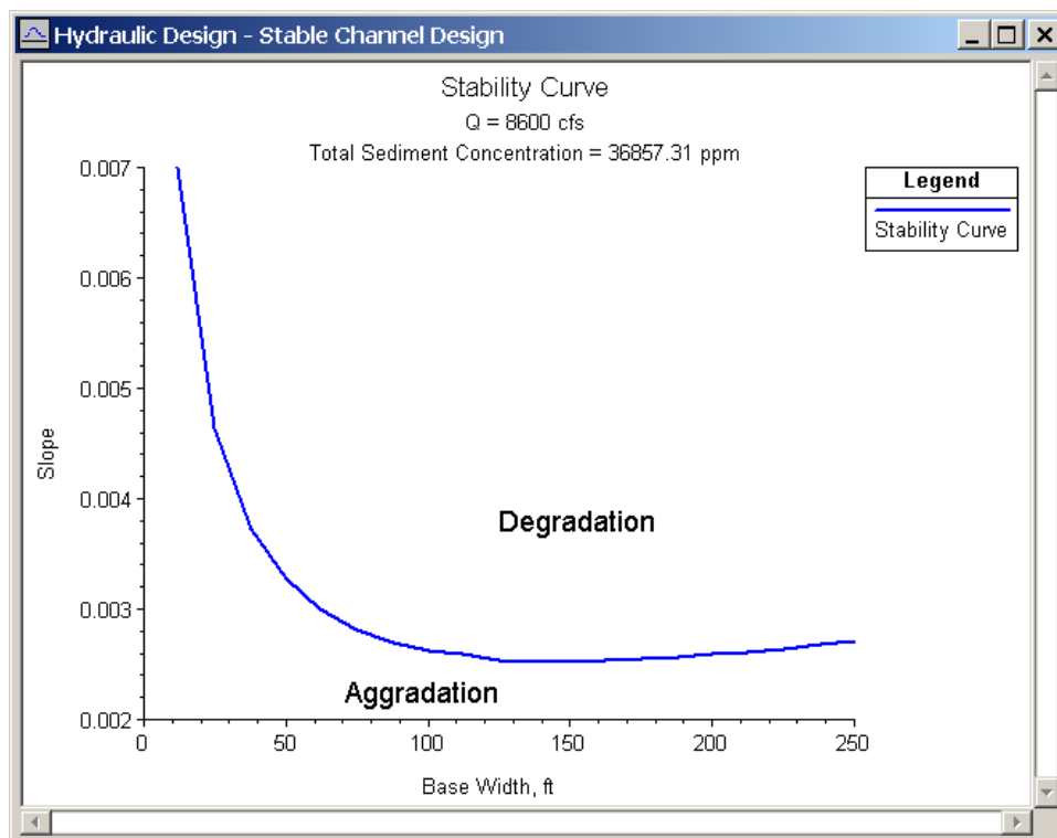
Figure 12-4 Stability Curve
