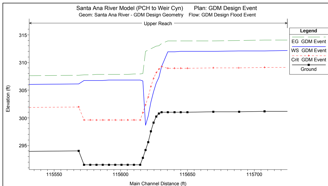
Figure 8-11 Drop Structure Modeled With Cross Sections
