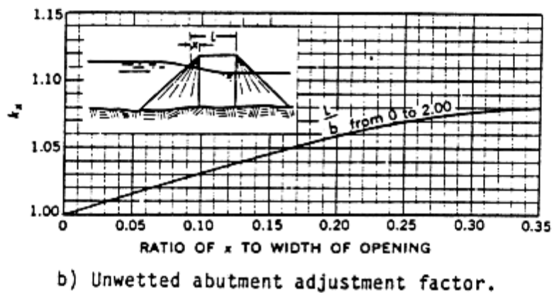
Figure D- 14 Coefficients for type 3 openings, embankment slope 2 to 1 (after Matthai)
